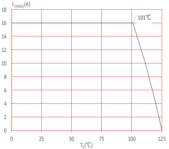
FIG.4: On-state characteristics
